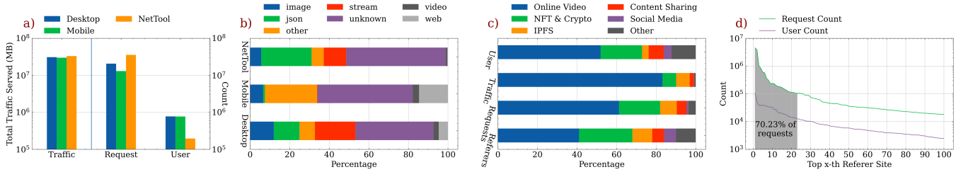
Figure 6: (a) Number of requests, number of unique users, and total traffic served for different user-agents; (b) Breakdown of requested file types for different user-agents; (c) Breakdown of referers for number of referral sites, the number of requests, total traffic served, and user count of the different referral types across the top 100 sites ranked by requests count; (d) The requests count and user count of the top 100 referer sites, ranked by request count and by user count, respectively.
