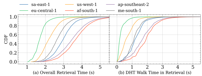
Figure 2: CDF for content retrieval for each AWS region: a) The overall retrieval duration, and b) the DHT walk.
