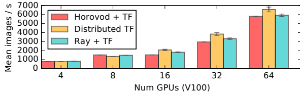
Figure 13: Images per second reached when distributing the training of a ResNet-101 TensorFlow model (from the official TF benchmark). All experiments were run on p3.16x1 instances connected by 25Gbps Ethernet, and workers allocated 4 GPUs per node as done in Horovod [53]. We note some measurement deviations from previously reported, likely due to hardware differences and recent TensorFlow performance improvements. We used OpenMPI 3.0, TF 1.8, and NCCL2 for all runs.
